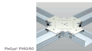
PlaGyp® PX60/60
